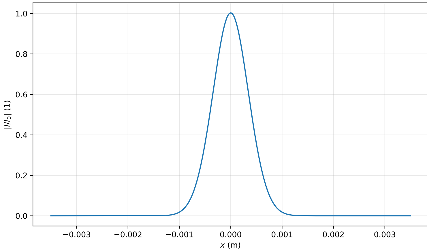
Intensity profile I(x, y = 0, z = 0.318m)/I_0 , P_{in}=0.3P_{cr} , artificial time
